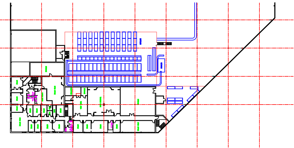
MEZZANINE PLAN
